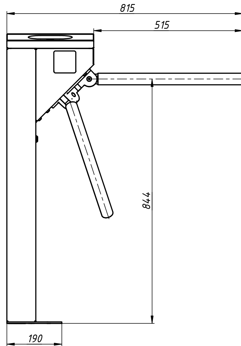
Installation tamplate
