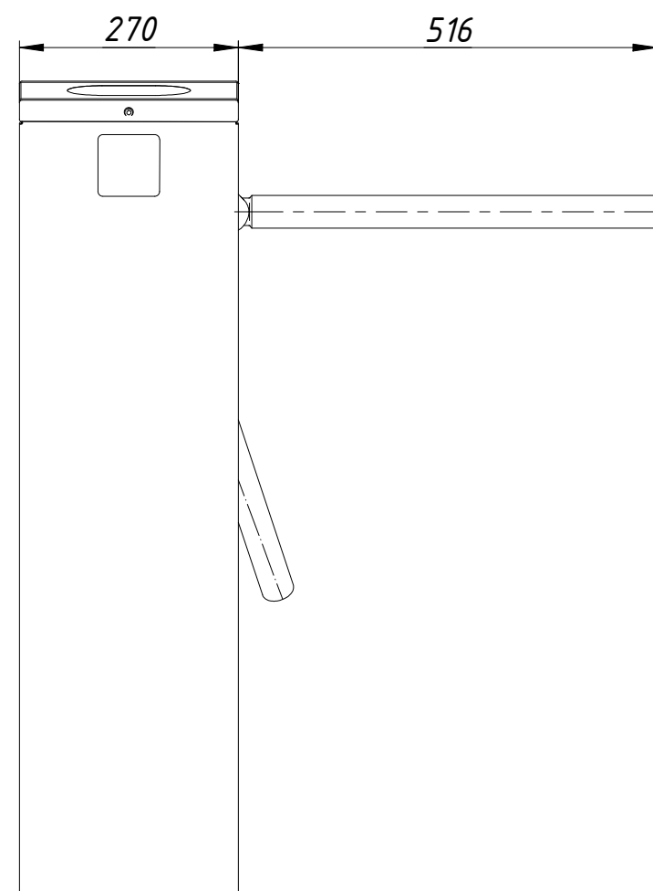
Instalation tamplate
