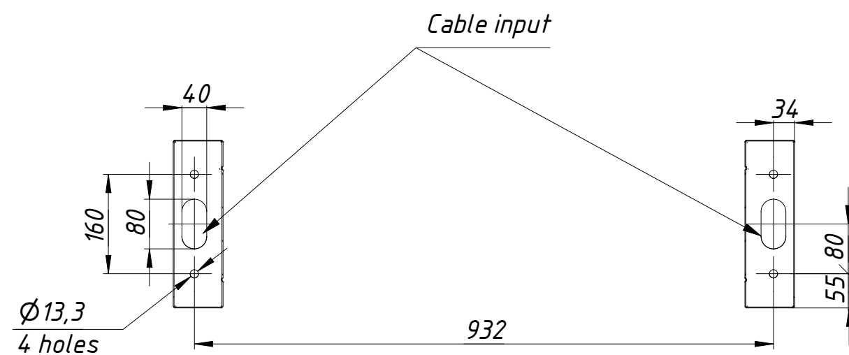
Instalation tamplate
