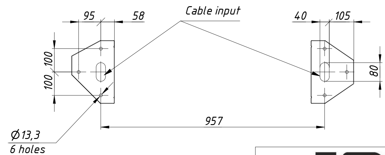
Installation tamplate
