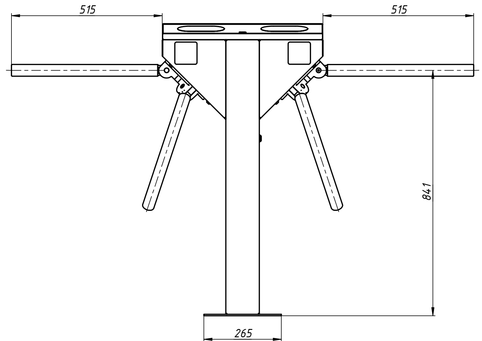
Installation tamplate
