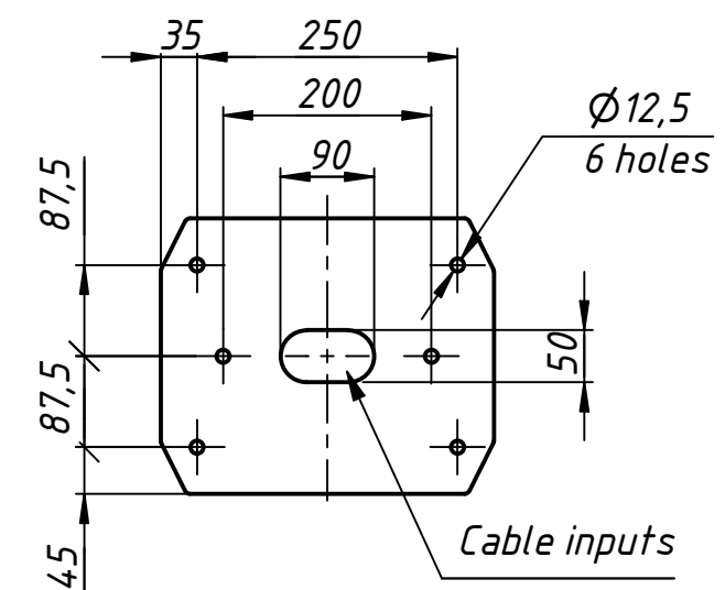
Installation tamplate
