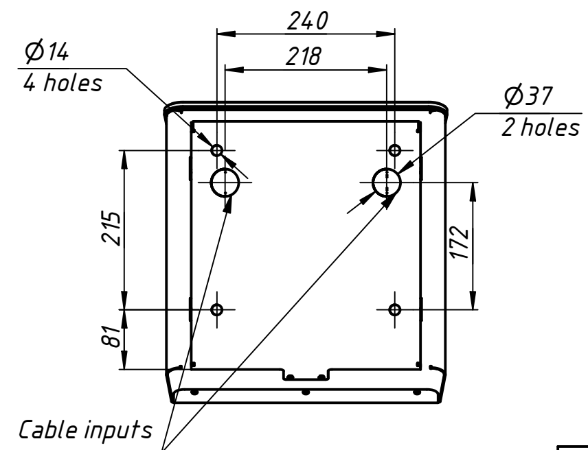
Instalation tamplate
