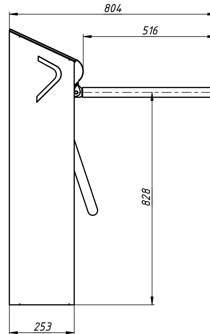
Installation tamplate
