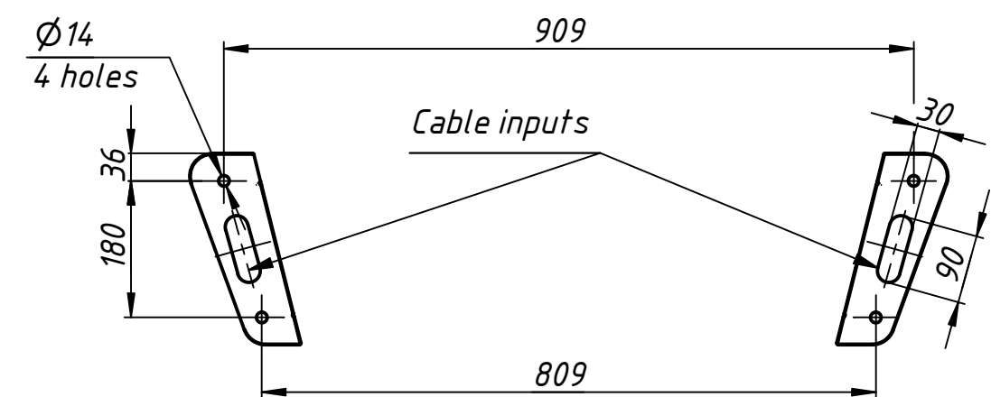
Installation tamplate
