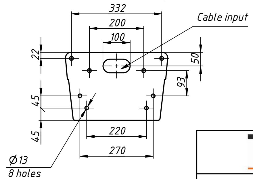
Instalation tamplate
