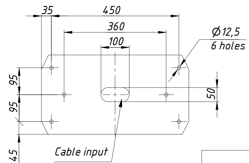
Installation tamplate
