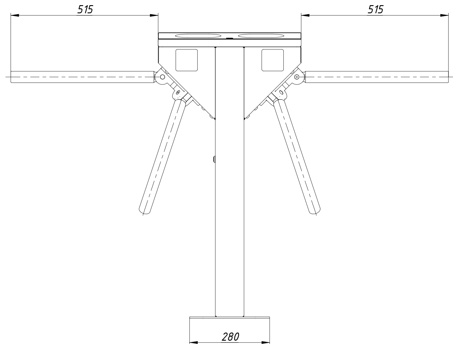
Installation tamplate
