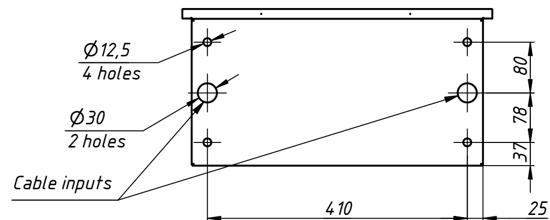
Instalation tamplate
